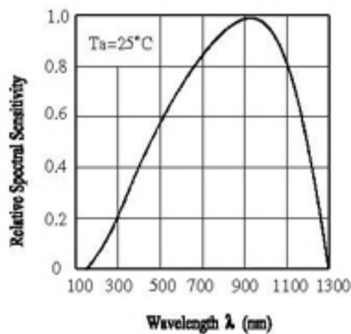
Fig.5 Spectral Sensitivity
