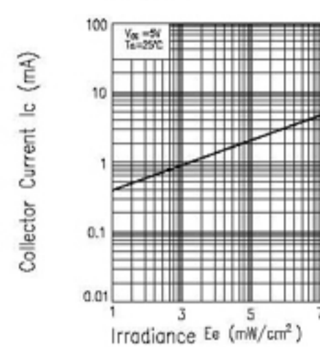
Fig.4 Collector Current vs. Irradiance
