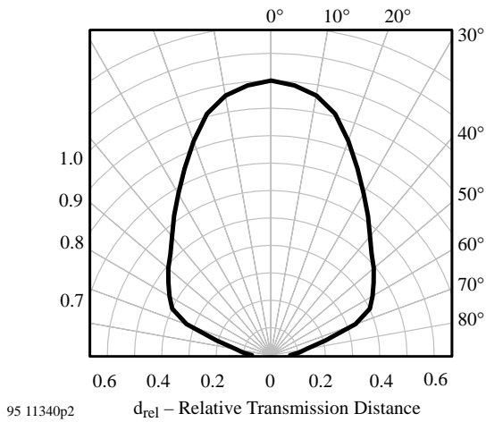
Figure 13. Horizontal Directivity \phi_x
